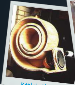
B&W Nautilus Prototype
